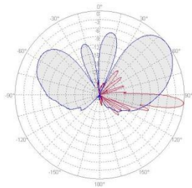
60 ° Service Beam
